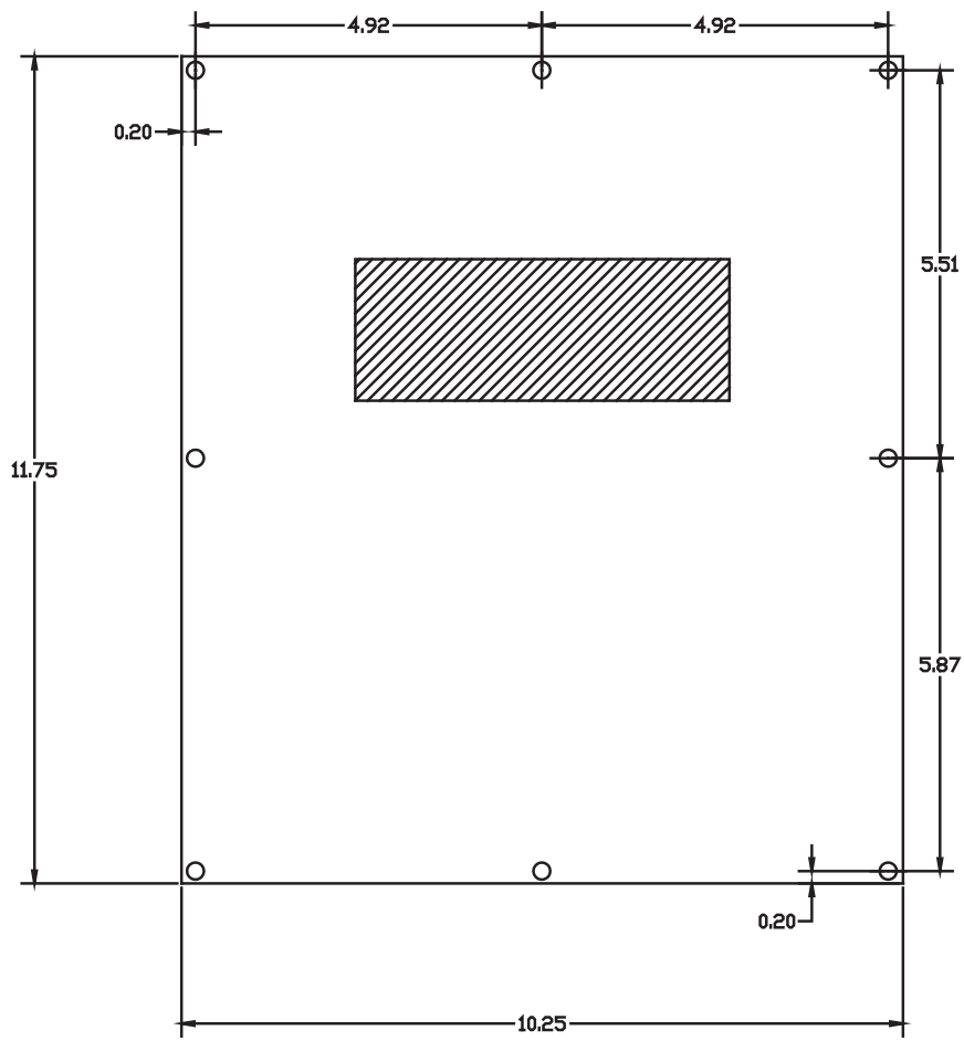
Controller Outline Dimensions (In Inches)
